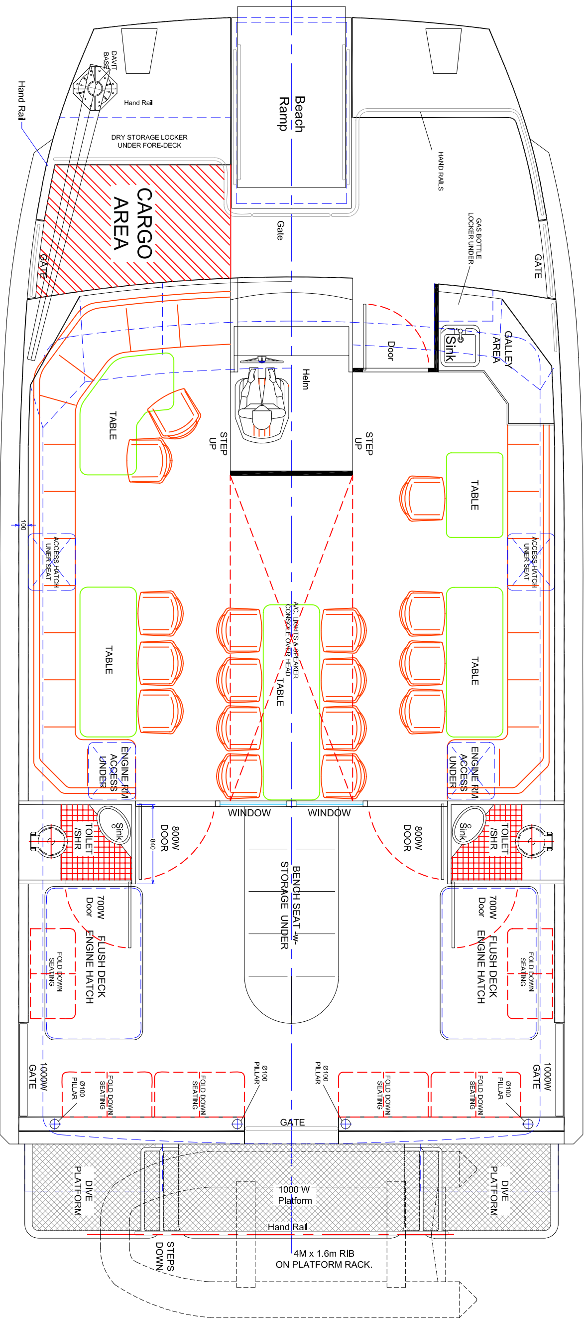
B F13 BHD 4 BHD 3 F12 F11 BHD 2 F9 F8 F7 BHD 1 F5 F4 F3 F2 F1 T Forward Compartment Toilet Compartment Engine Compartment Tiller Compartment Main Deck Plan
